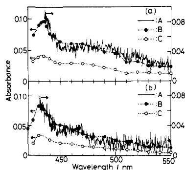
Figure 6. Time-resolved absorption spectra of CN-NO 2 -A (a) and Bz-NO 2 -A (b) in benzene at room temperature. A, at 460-ps delay by picosecond laser photolysis; B and C, at 50-ns and 10- \mu s delays by nanosecond laser photolysis, respectively.
