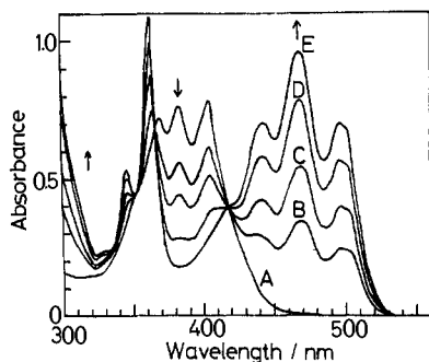
Figure 1. Absorption spectral change of CN-NO 2 -A in basic ethanol upon irradiation at room temperature. A, 0; B, 0.5; C, 1.0; D, 2.0; E, 4.0 min.
